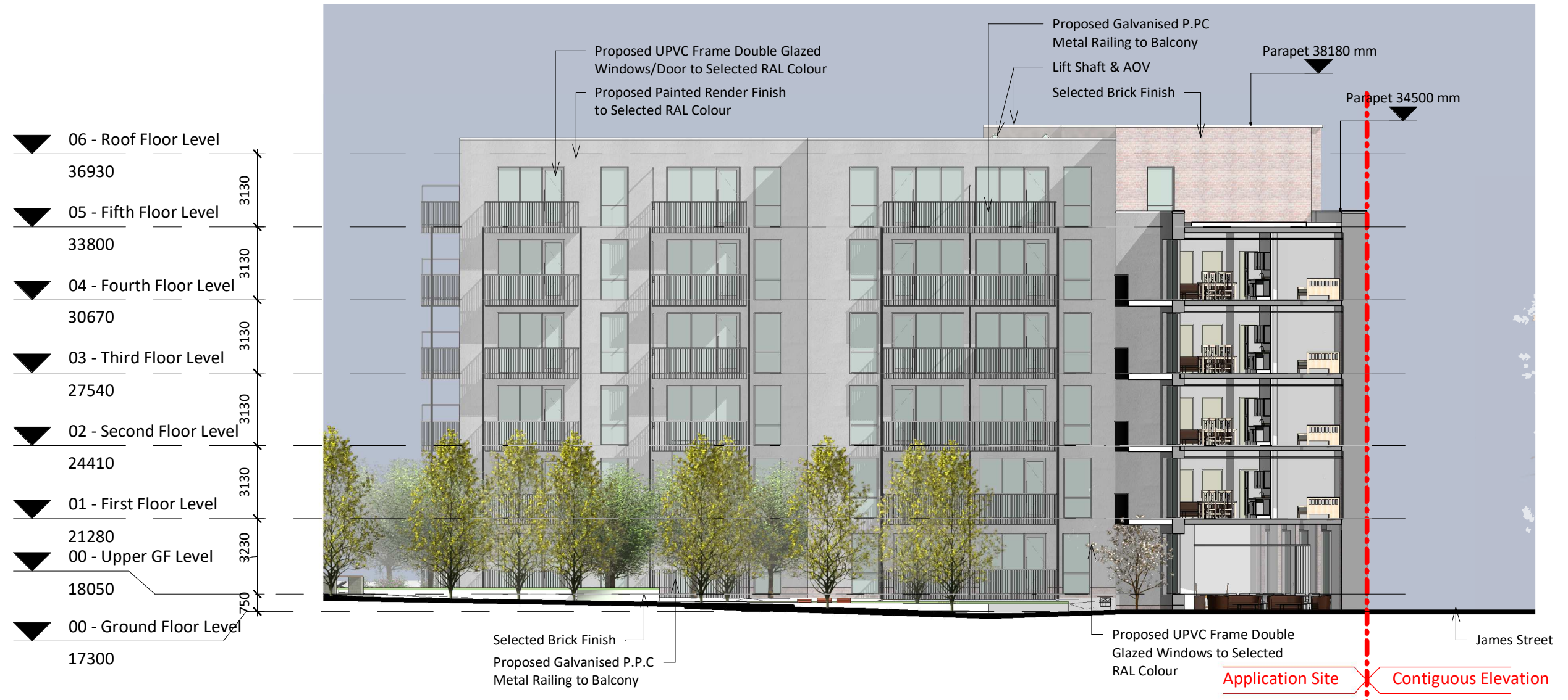
1 Elevation - East 1 : 200
