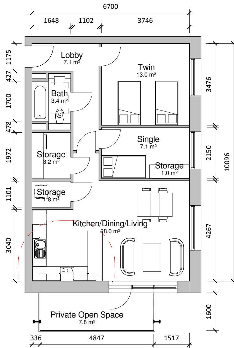
1 2 Bed/3P - 67.6sqm 1 : 100
